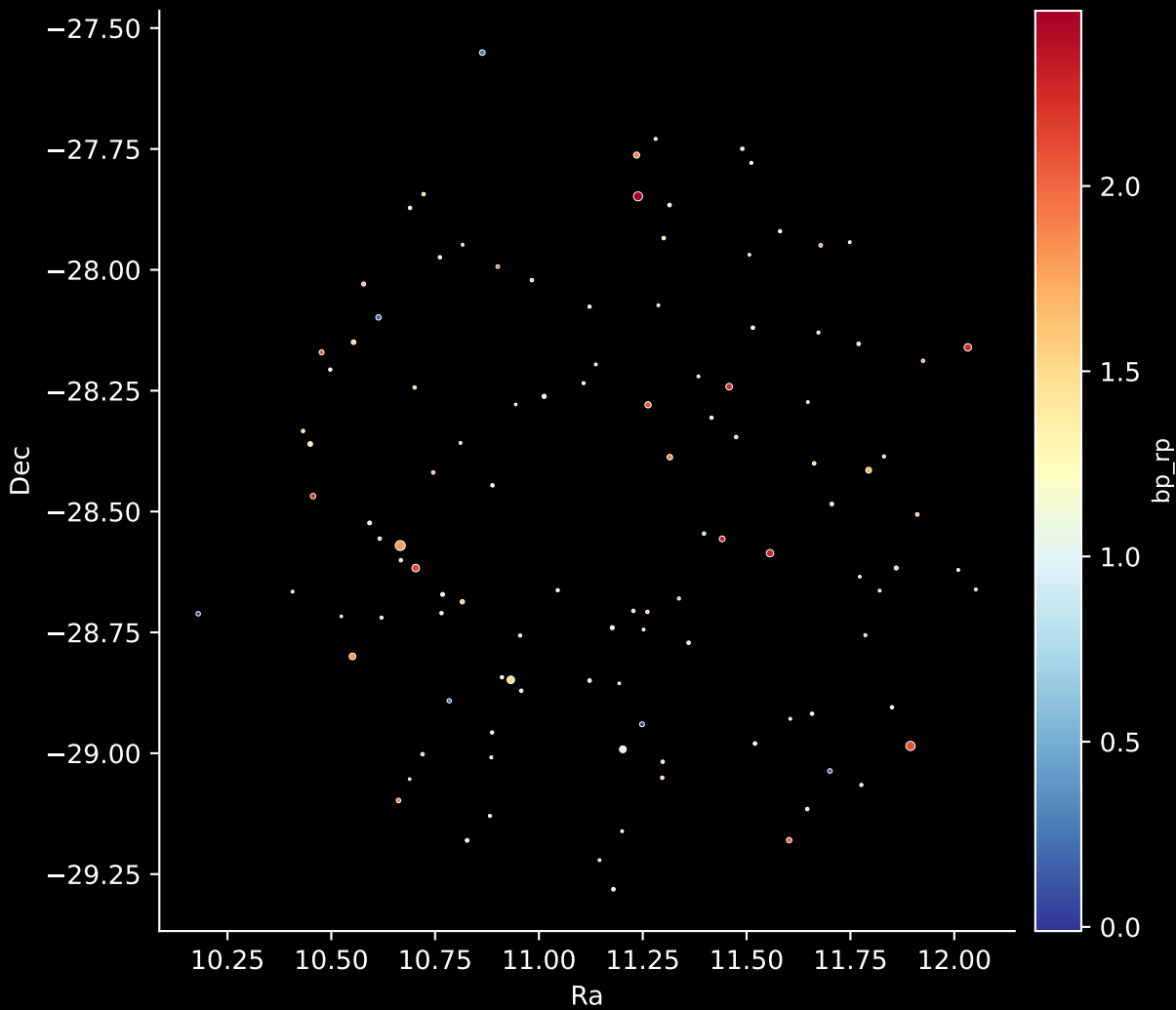
APOGEE DR17 Field: [003-03-O] Stars: 112
