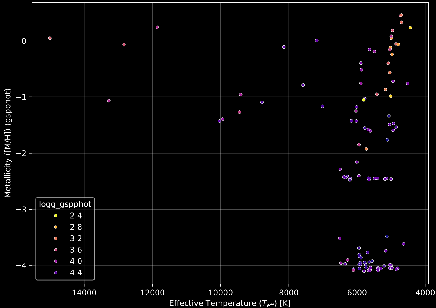
APOGEE DR17 Field: [003-03-O] Stellar Population Parameters (n= 112)
