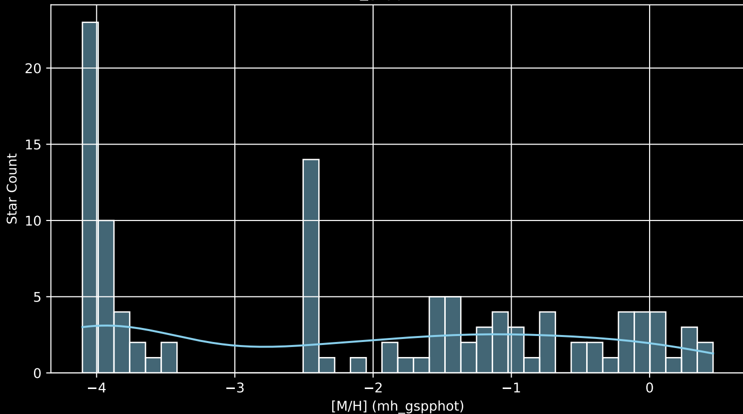
APOGEE DR17 Field: [003-03-O [M/H] (mh_gspphot) (n= 112)
