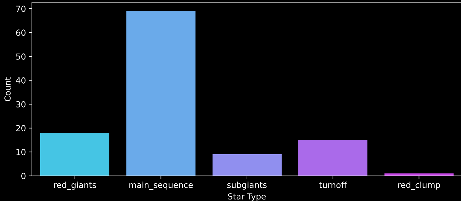
APOGEE DR17 Field: [003-03-O] Count plot of Star Type
